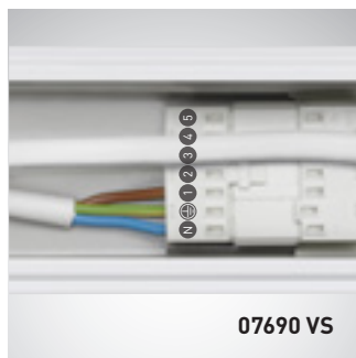
7-pole plug for infeed, rigid
