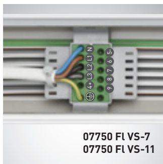
7 or 11-pole plug for infeed, rigid
